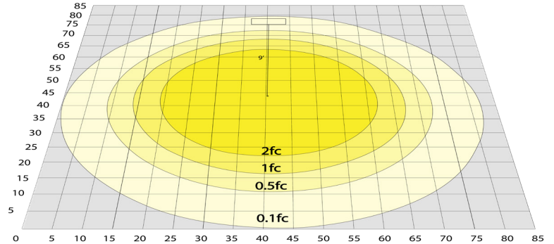
Simulation based on 4000K Area 85'x 85' Mounting Height: 9'
